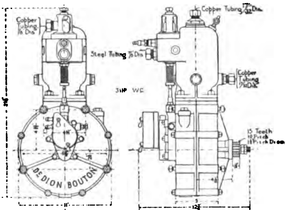
FIG. 260.—Rear and Side Elevation of a De Dion Water-Cooled Carriage Motor, showing method of joining the two halves of the crank case and bolting them to the cylinder. As indicated, also, the water-jackets, cylinder head and valve chamber are cast integral with the cylinder.
